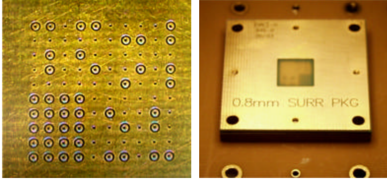
Figure 2 : Fixture showing Probe Side (left) and Socket/ Interconnect Side with sample (right)
