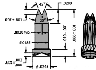
92-30715-2 Ø .0185 w/ Ø .0245 Base BGA Crown Hardhat
