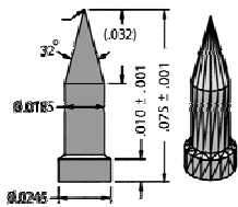
92-30707 Ø .020 w/ Sharp Tapered Tip Hardhat
