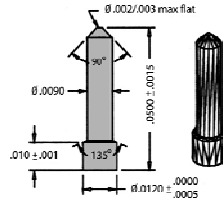
92-30722 Dia .010 Tapered Tip Hardhat
