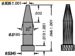
92-30737 Ø .006 Flat Tapered Tip Hardhat
