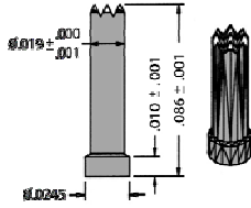
92-30711 Ø .020 x .086L LGA Serrated Hardhat
