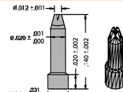
92-30053 Ø .030 BGA Crown Hardhat
