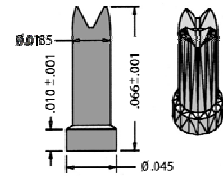
92-30045 Ø .020 BGA Crown Hardhat
