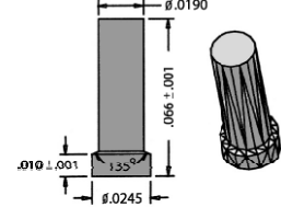
92-30728 Ø .020 LGA Flat Top Hardhat
