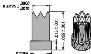
92-30048-1 Ø .030 LGA Serrated Hardhat
