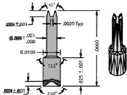
92-30730 Ø .009 W/ Ø .015 Base BGA Crown Hardhat
