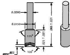
92-30742 Ø .009 W/ Ø .015 Base Flat Top Hardhat
