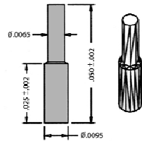
92-30051 Dia .010 LGA/BGA Flat Top Hardhat
