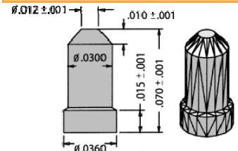
92-30090 Ø .012 Flat Tapered Tip Hardhat
