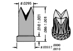
92-30703 Ø .030 x .086L BGA Crown Hardhat
