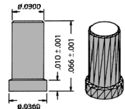
92-30719 Ø .030 Flat Top Hardhat
