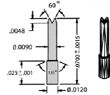
92-30723 Dia .010 BGA Crown Hardhat
