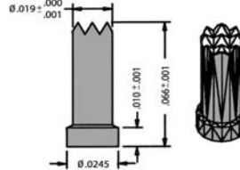
92-30028-5 Ø .020 LGA Serrated Hardhat
