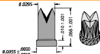
92-30033-2 Ø .030 BGA Crown Hardhat
