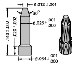
92-30060 Ø .030 LGA Tapered Tip Hardhat
