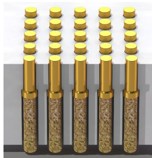
Cross-section of socket
